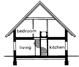
7 Section, small house without basement → 8 + 9
